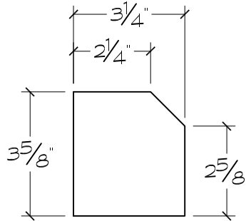
CROSS SECTION
